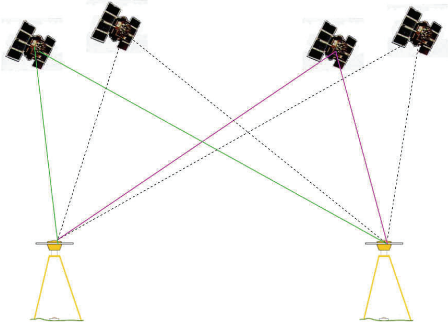
Triple difference – difference of two double differences at two epochs for two satellites and two receivers
