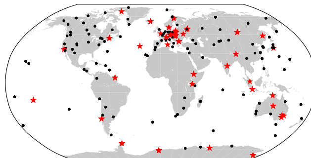
(c) GNSS subnetwork of the IGS in April 2008 (day of year 110)
