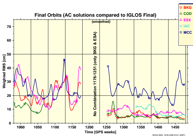
Figure 6: Consistency of the GLONASS orbits in the combination procedure ( http://www.ngs.noaa.gov/igsacc/www/ ). (The MCC solution is based on SLR data for only three GLONASS satellites.)
