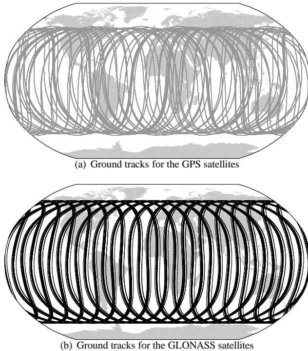
Figure 10: Ground tracks of the GPS (top) and GLONASS (bottom) constellation for 10 days (day 60 to 69 of year 2008) in February 2008.
