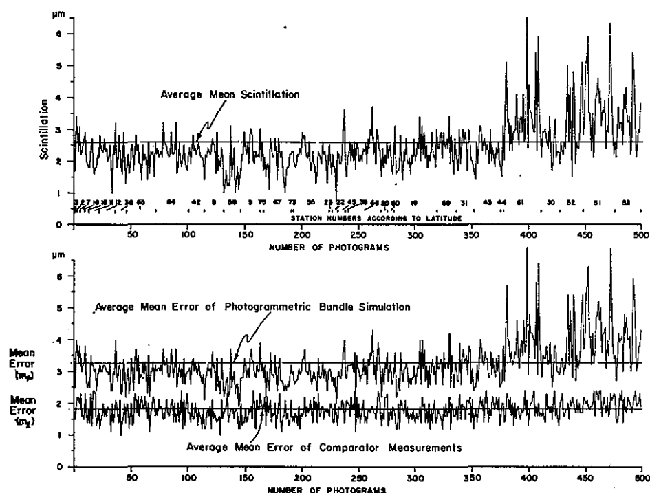
Figure 40.—500 photograms, arranged according to increasing latitude of observing station, showing, in the top diagram, the amount of scintillation for each plate and, below, the mean errors of the bundle simulation and the comparator measurements, respectively.
