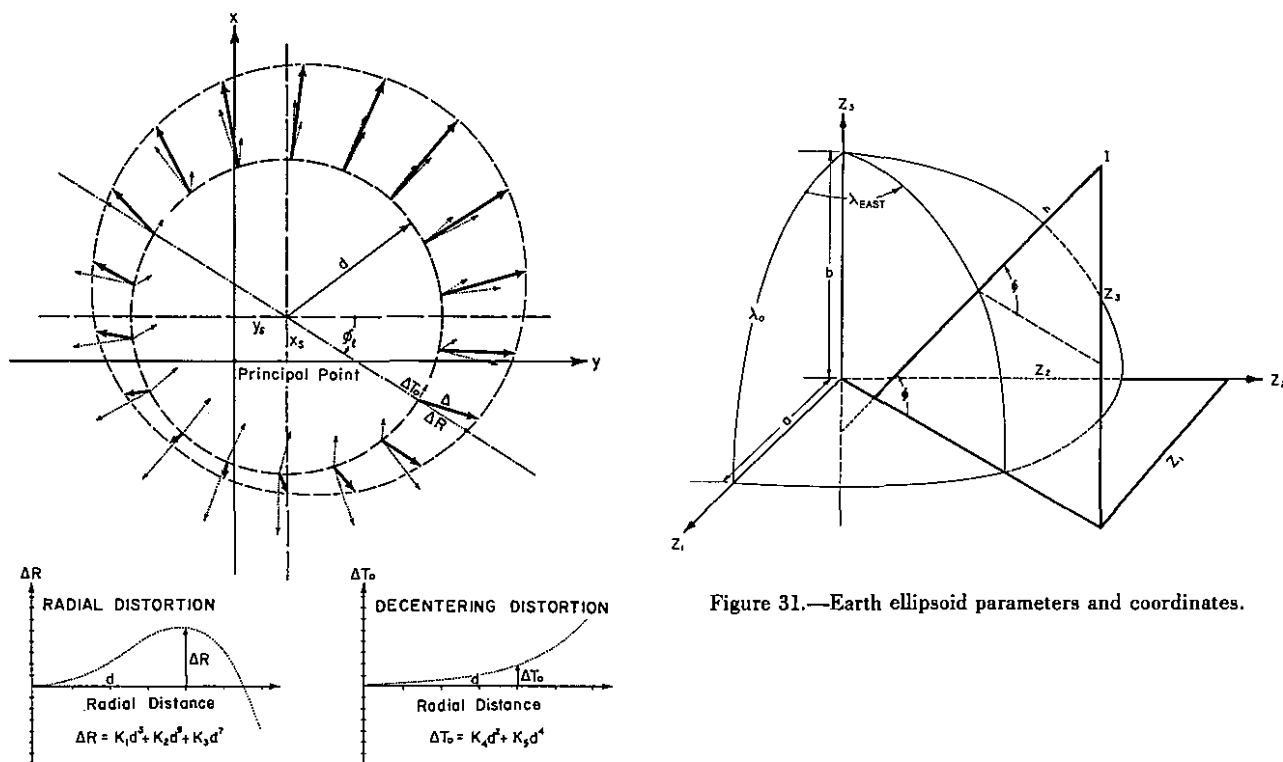
Figure 30.—Components of distortion.
