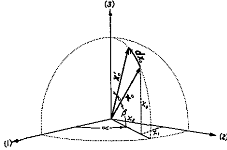
Figure 26.—Increment coplanar with a coordinate axis.
