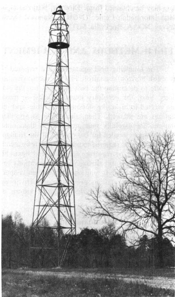
Figure 1b.—Completed tower
