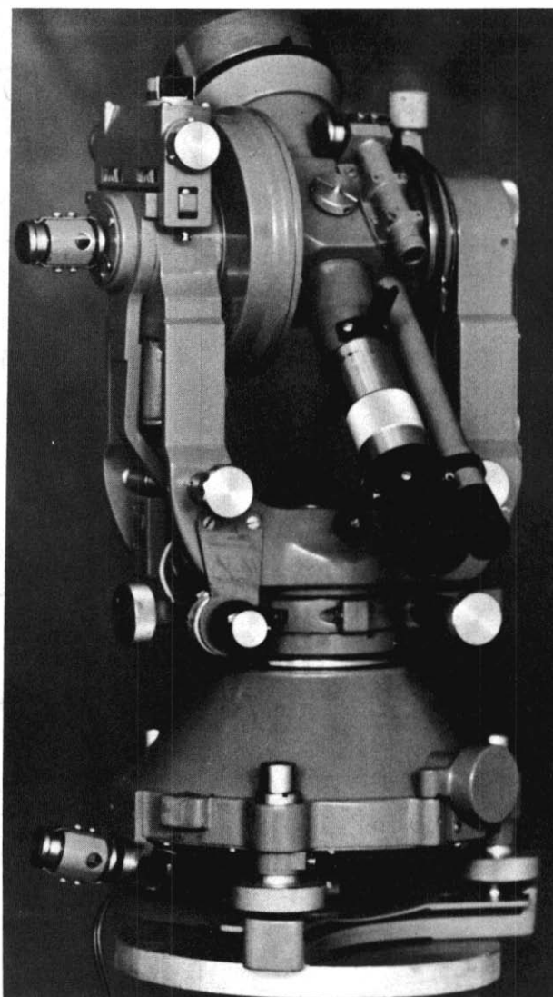
Figure 4.—Wild T-3 theodolite
