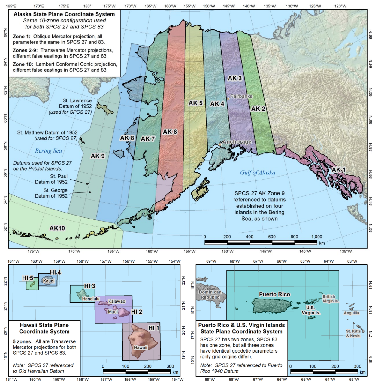
Figure 3. Zones of the State Plane Coordinate Systems of 1927 and 1983 for Alaska, Hawaii, and Puerto Rico and the U.S. Virgin Islands.
