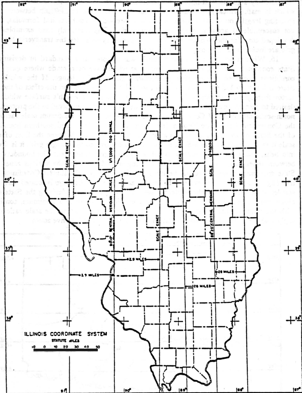
FIGURE 4.—The Illinois Coordinate System
