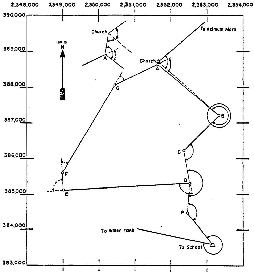
FIGURE 18.—Plat of farm survey
