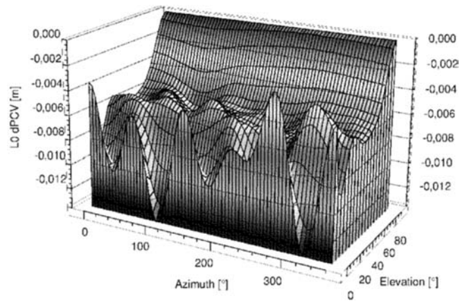
Fig. 16 Differences of absolute L0 PCVs for AT504 with LEIS or SCIS
