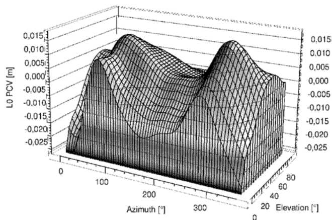
Fig. 6 Absolute L0 PCV of CZJRD24* integrated antenna/receiver system
