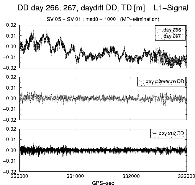
Fig. 1 Elimination of Multipath
