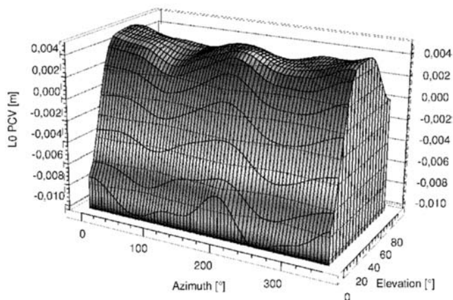
Fig. 23 Absolute L0 PCV for JPSLEGANT
