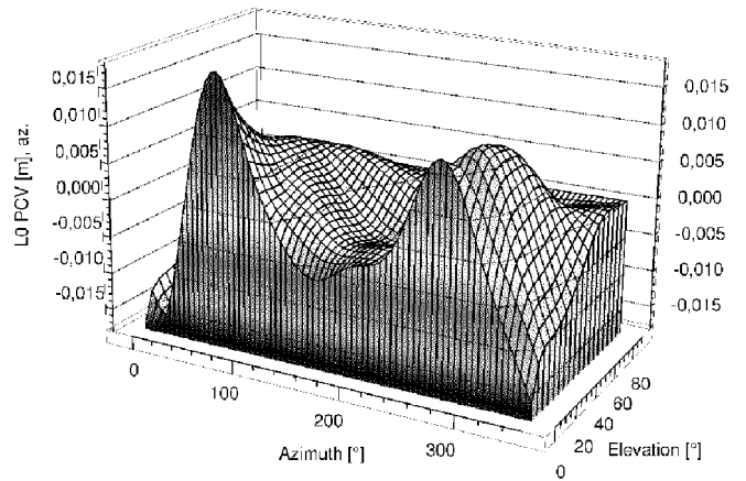
Fig. 7 Pure azimuthal L0 PCV of CZJRD24* integrated antenna/receiver system
