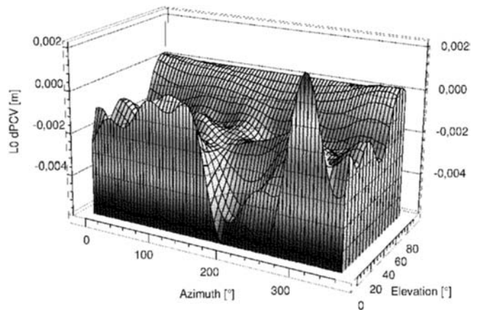
Fig. 17 Differences of absolute L0 PCVs of LEIAT504 with and without LEIS
