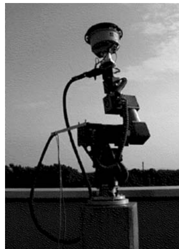
Fig. 9 TRM4800 during absolute calibration on the robot
