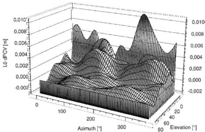
Fig. 14 Differences of absolute L0 PCV for LEIAT303 with and without LEIC dome (elevations from 90 to 0°)
