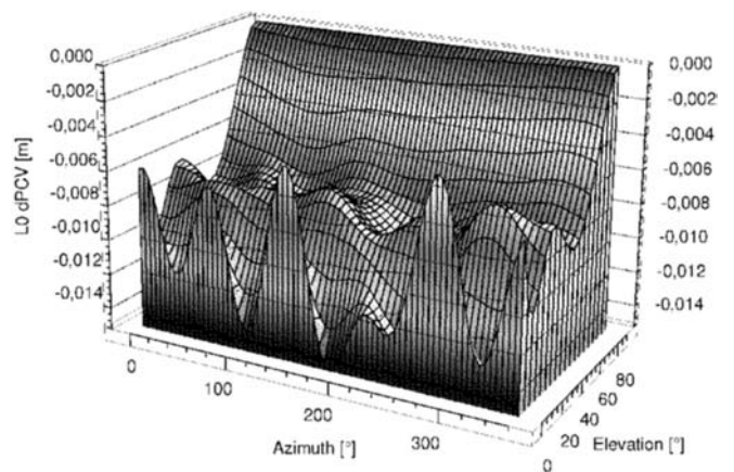
Fig. 18 Differences of absolute L0 PCVs of LEIAT504 with and without SCIS
