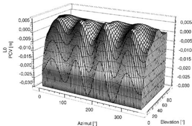
Fig. 19 Absolute L0 PCV for TRM22020.00 without ground plane
