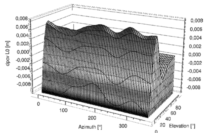
Fig. 12 Differences of absolute L0 PCV for TRM29659.00 with and without TCWD
