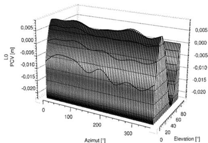
Fig. 20 Absolute L0 PCV for TRM22020.00 with ground plane
