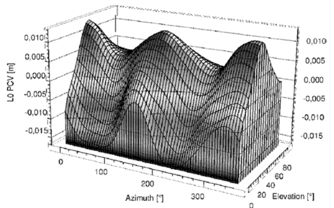
Fig. 2 Absolute L0 PCV with LEIAT303_LEIC
