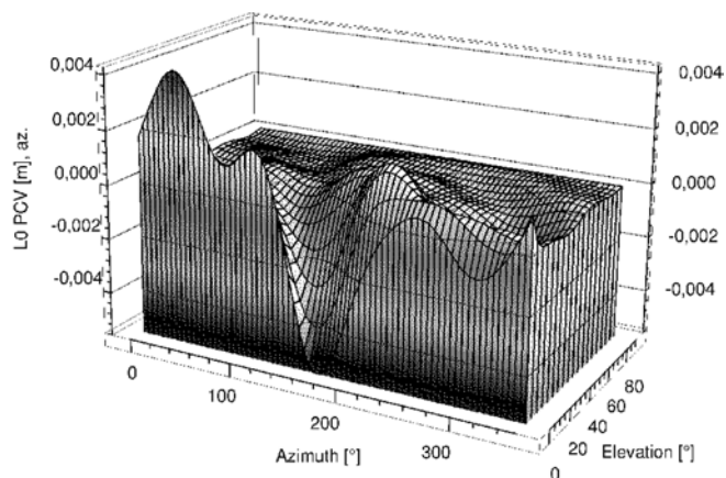
Fig. 11 Pure azimuthal L0 PCV of TRM4800 integrated antenna/receiver system
