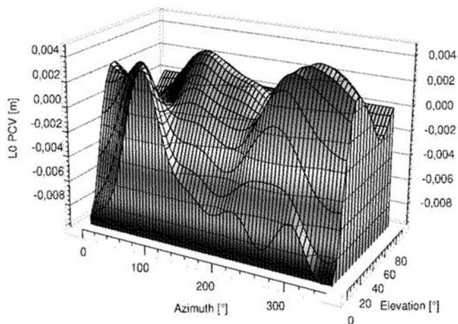
Fig. 24 Absolute L0 PCV for DSNAP_002*
