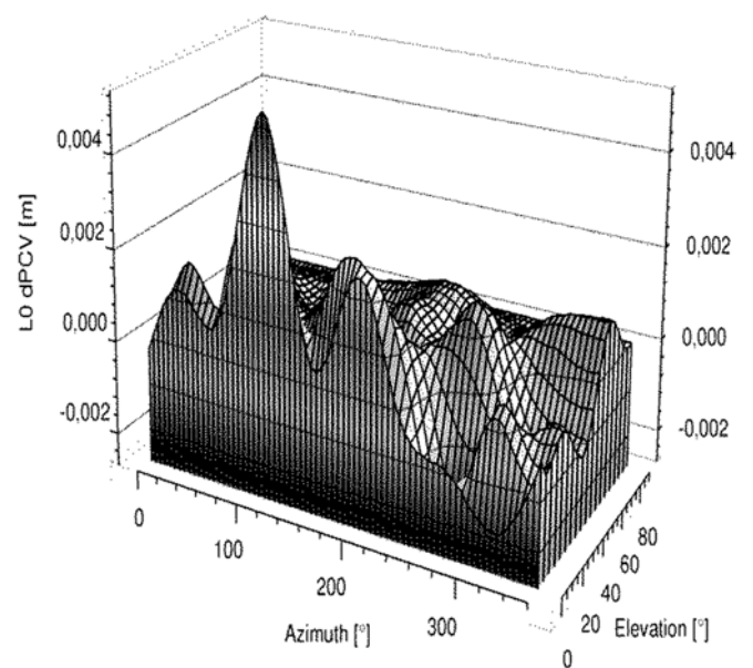
Fig. 3 Difference of two L0 PCV LEIAT303_LEIC calibrations, 5 months
