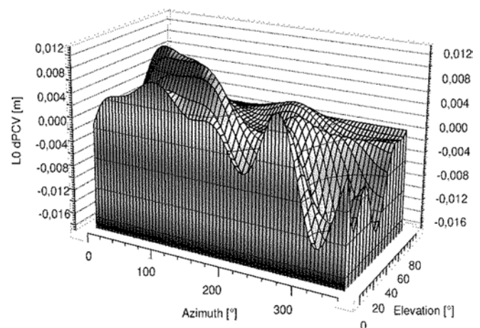
Fig. 5 Absolute L0 PCV differences for DSNDGU_002* with and without passive UHF aerial
