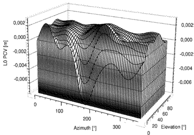
Fig. 10 Absolute L0 PCV of TRM4800 integrated antenna/receiver system
