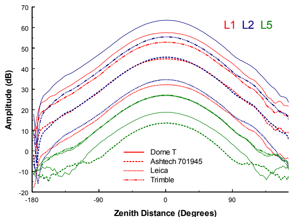
Figure 3 - The Amplitude Response of 4 Choking GPS Antennas at L1, L2, and L5
