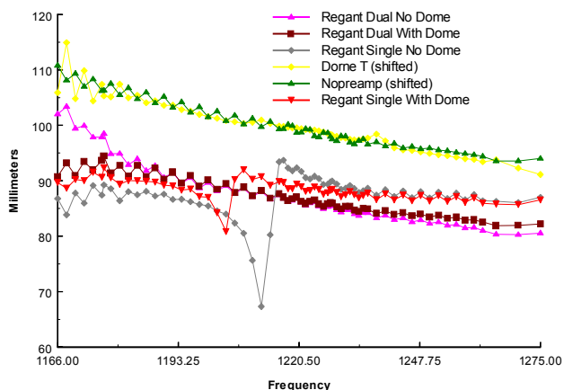
Figure 9 - The Vertical Phase Center Position of the JPS Antennas as Compared to the Dorne T at L2 and L5
