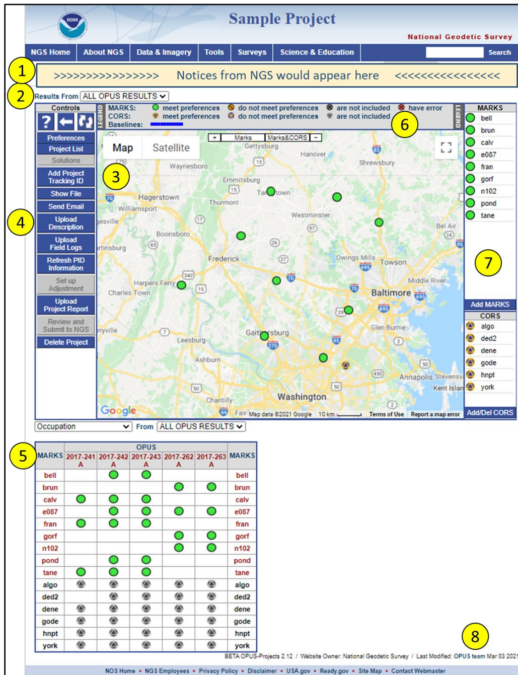
Figure 7-1: The Project Manager's web page
