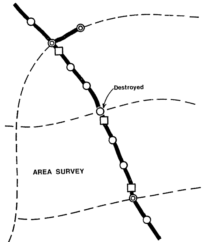
Figure 2-14.—Connections to an area survey.
