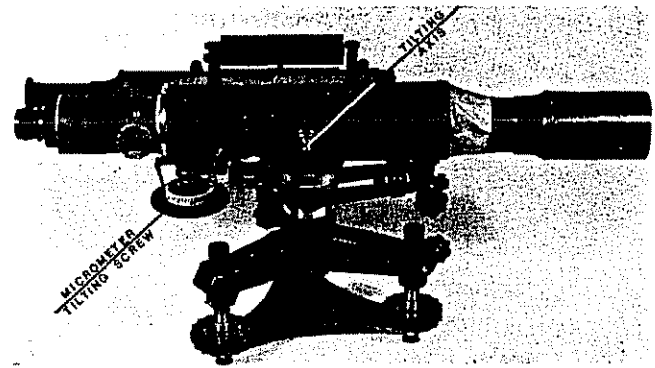
Figure 3-16.—Fischer level.
