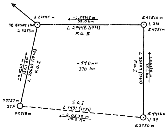
Figure 5-16.—Sample sketch for checking a loop.
