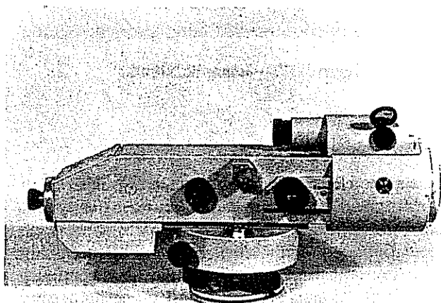
Figure 3-19.—Zeiss Ni1.
