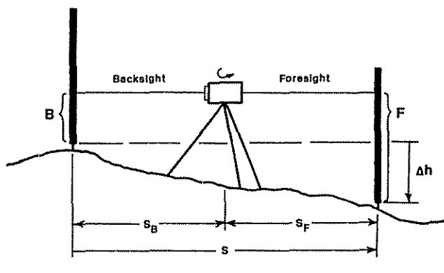
Figure 3-1.—Setup of leveling, \Delta h = B - F and s = s_B + s_F
