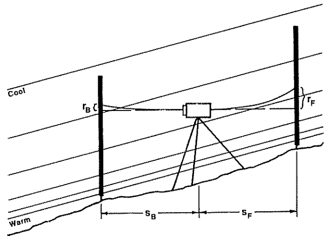
Figure 3-7.—Refraction error, r , does not cancel on sloping terrain since r_B \neq r_F , even if s_B = s_F .
