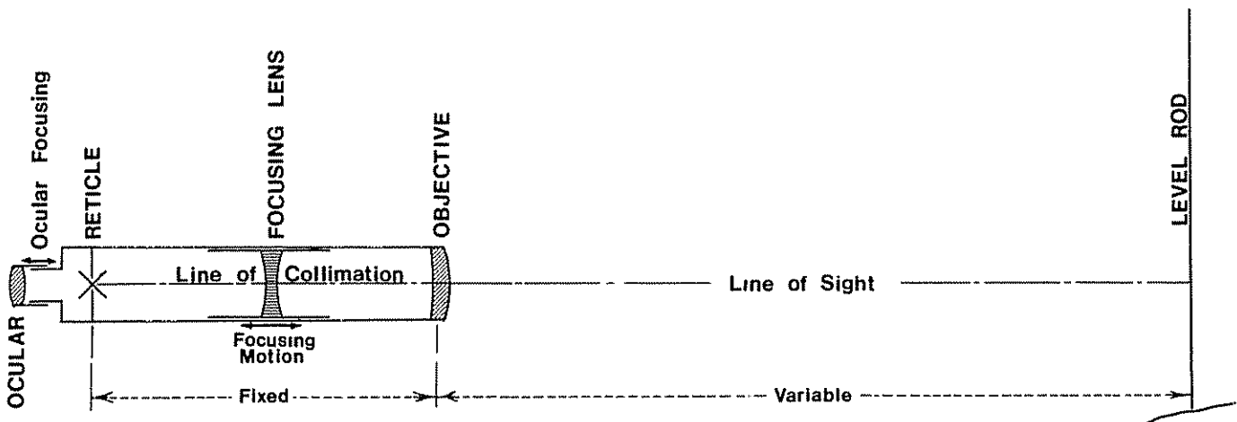
Figure 3-23.—Internal-focusing telescope.
