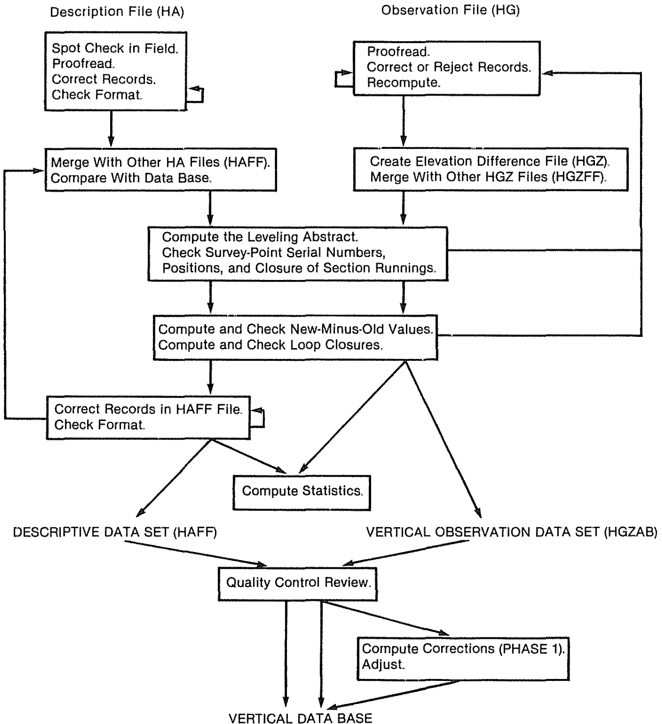
Figure 5-4.—Flow chart of project data processing.
