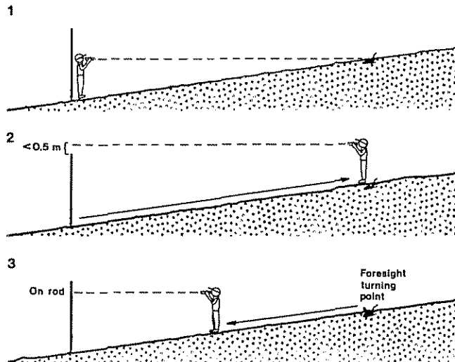
Figure 3-67.—Pacing a balanced setup on a slope.
