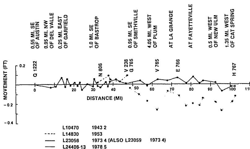
Figure 5-19.—Sample profile of a leveling line.
