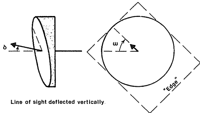
Figure 4-6.—Rotary wedge, unrotated (a) and rotated (b).
