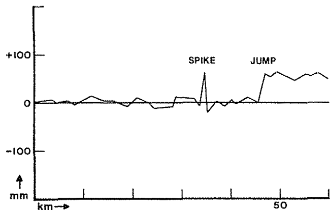
Figure 5-15.—Sample plot of new-minus-old values for observed elevations.
