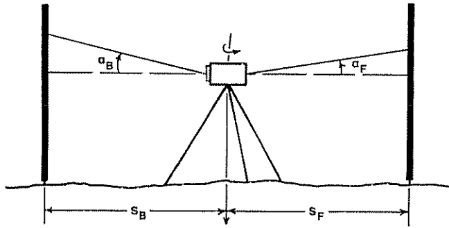
Figure 3-5.—Inconsistent collimation error does not cancel in a balanced setup since \alpha_B \neq \alpha_F , even if s_B = s_F .
