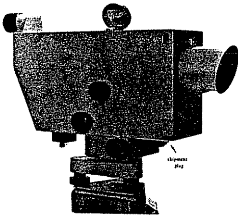
Figure 3-21.—Jenoptik NI 002.
