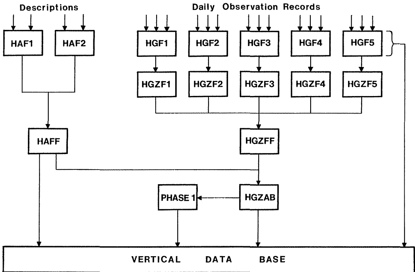
Figure 5-5.—Flow chart of data files for a line of leveling.
