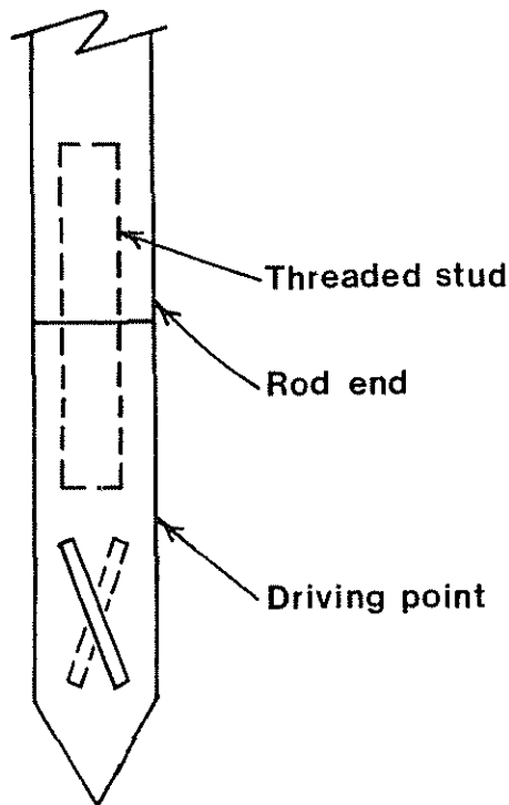
Figure 2-18.—Driving point for a rod mark.
