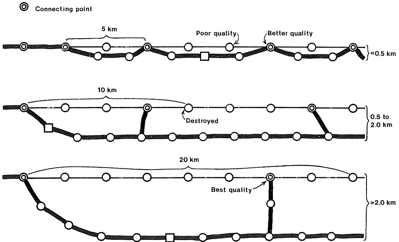
Figure 2-12.—Connections to parallel surveys.
