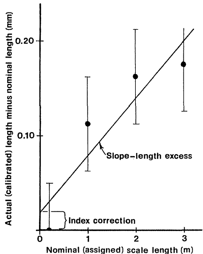
Figure 3-58.—Rod calibration data.
