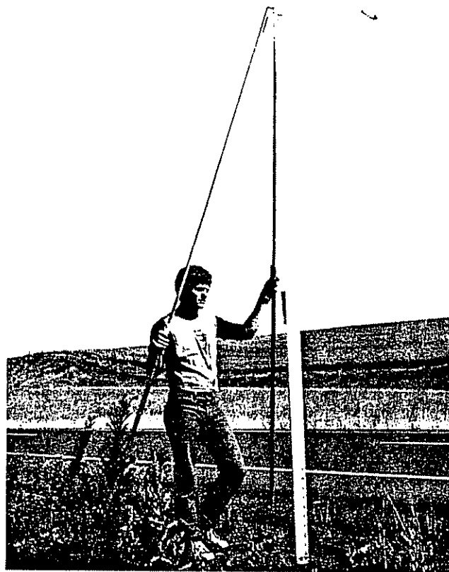
Figure 3-61.—Setup of leveling rod.
