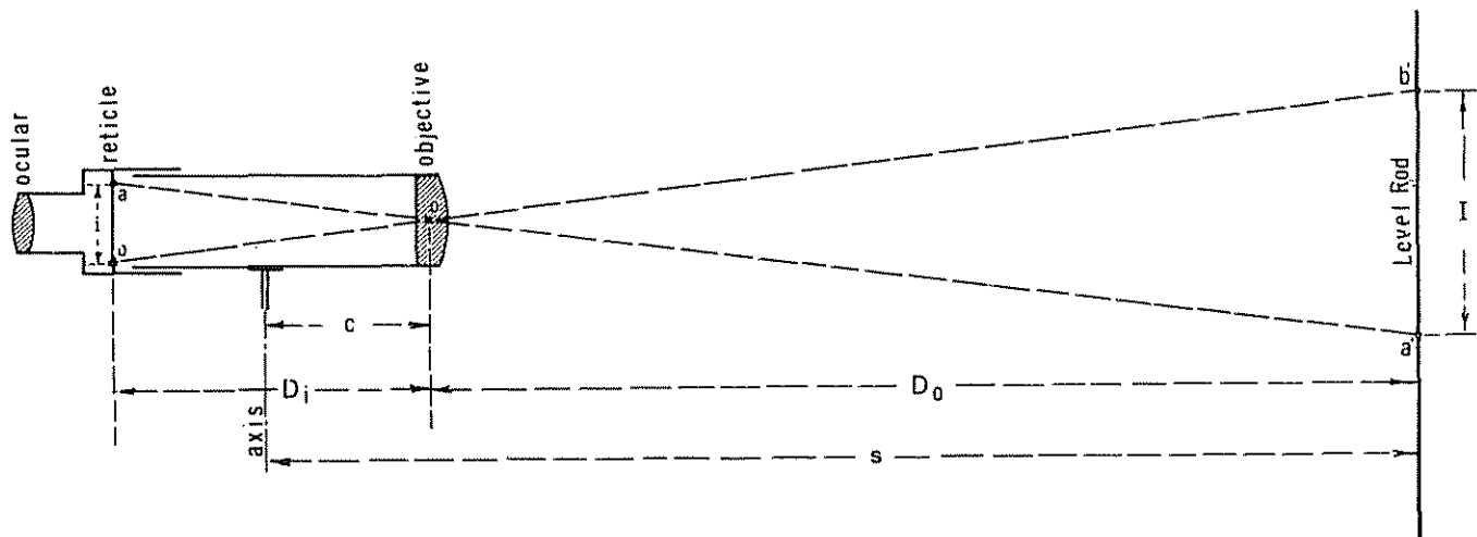
Figure 3-40.—Relationship of stadia interval to sighting distance.
