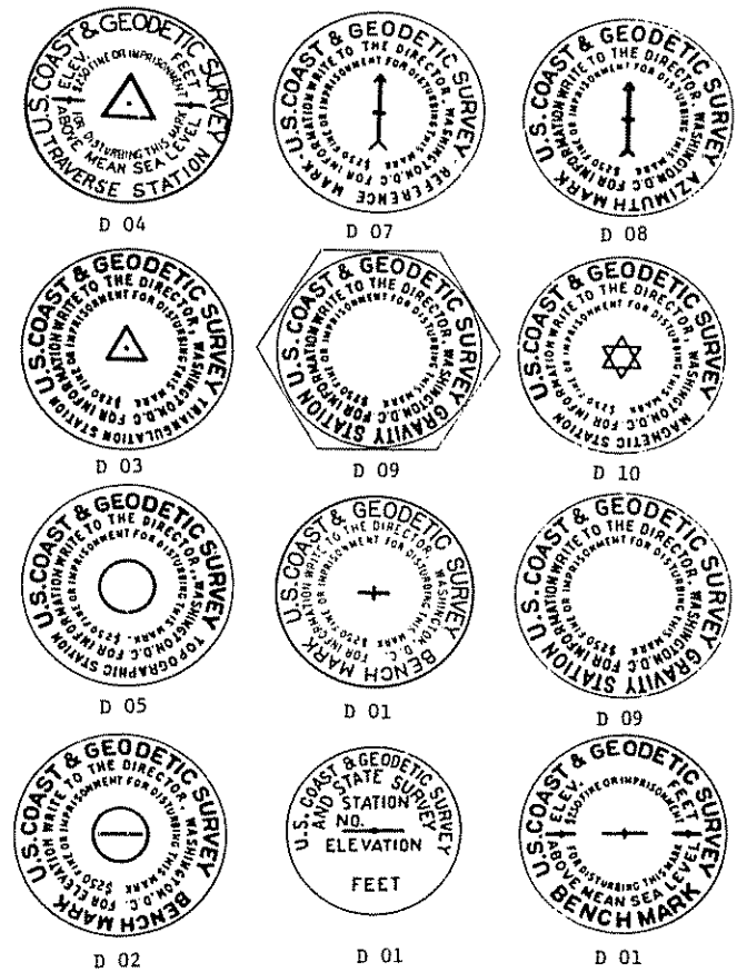
Figure 2-26.—Survey disks of the former U.S. Coast and Geodetic Survey.
