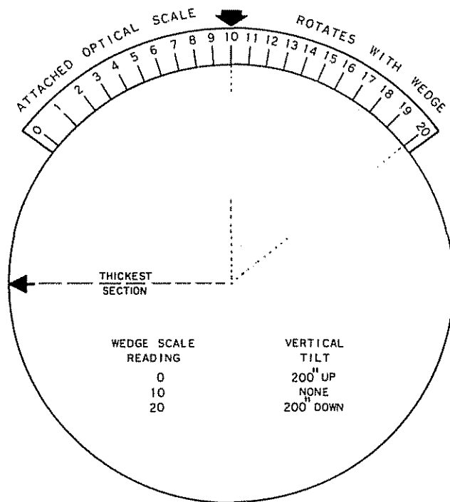
Figure 4-7.—Rotary wedge scale.
