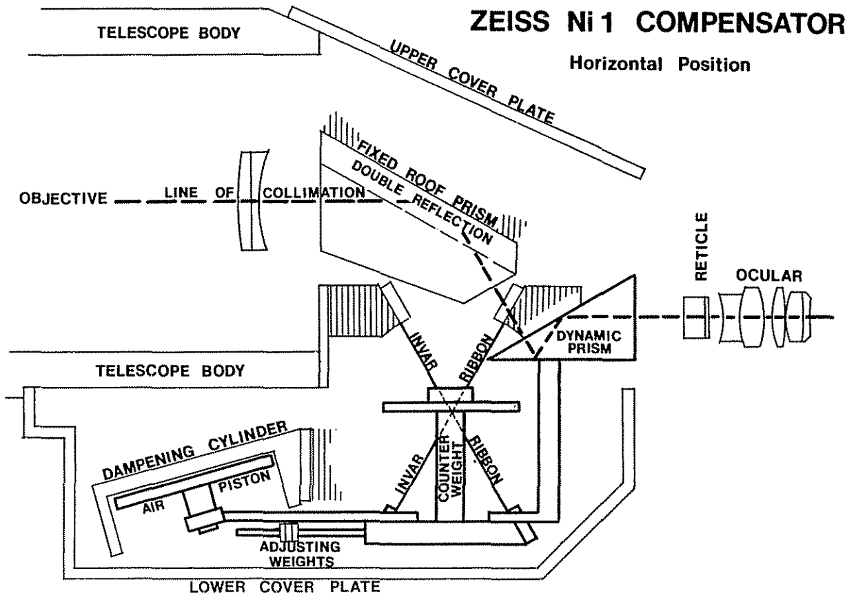
Figure 3-28.—Ni1 compensator system, telescope axis horizontal.
