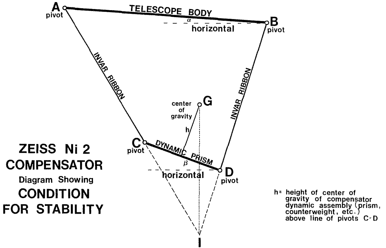
Figure 3-27.—Condition for dynamic stability of the Ni2.
