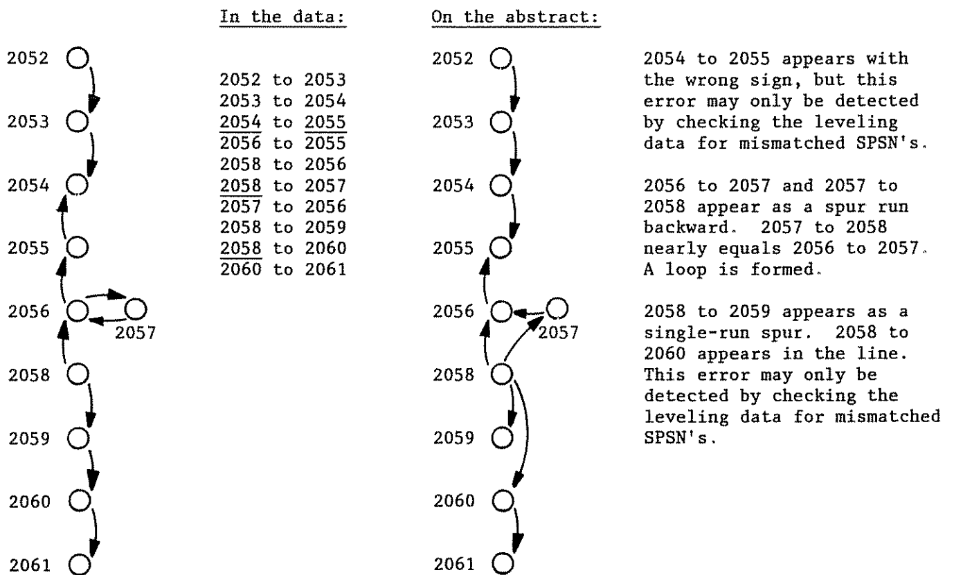
Figure 5-13.—Samples of incorrect survey-point serial numbers. Mismatched survey-point serial numbers are underlined.
