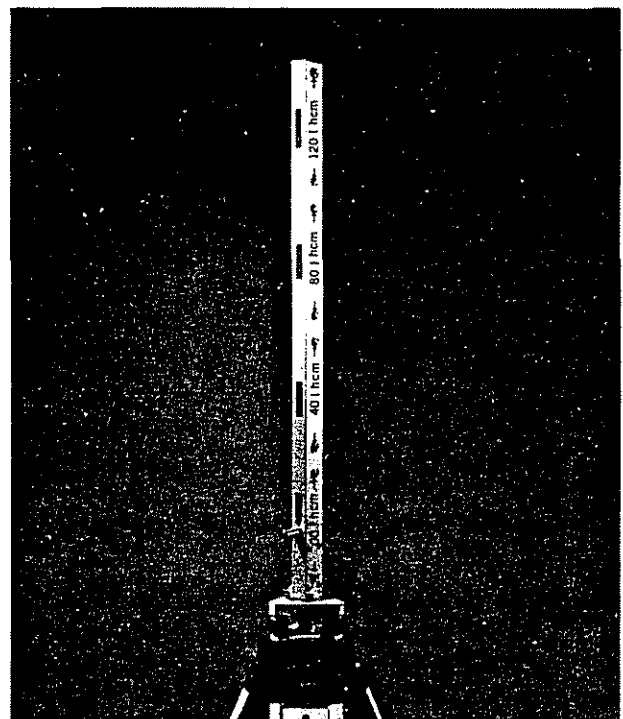
Figure 4-8.—Target column.
