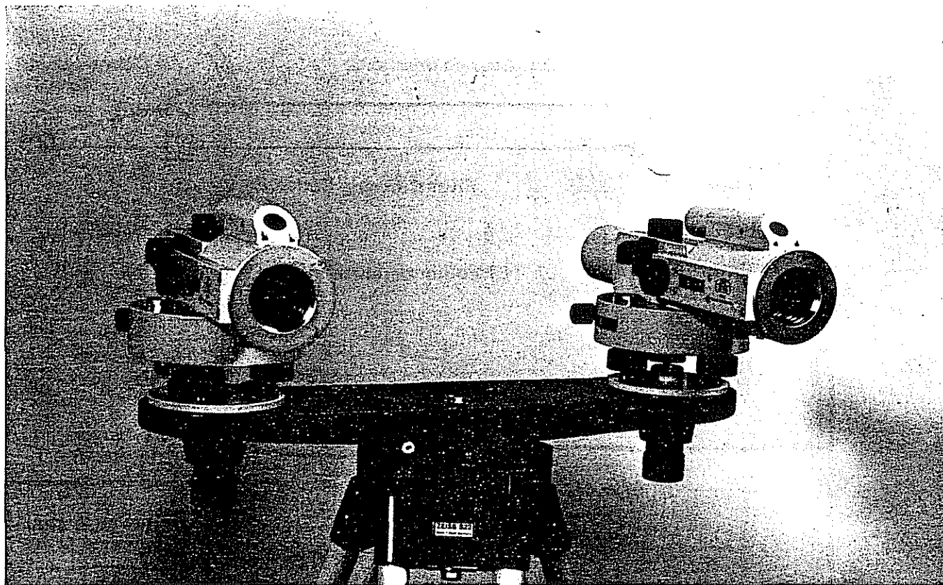
Figure 4-12.—Instruments mounted on base plate.
