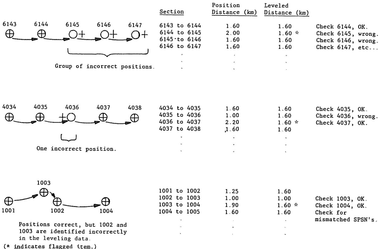
Figure 5-9.—Examples of apparent position errors.
