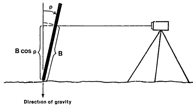
Figure 3-10.—Effect of rod plumbing error, \rho , on a height observation, B .
