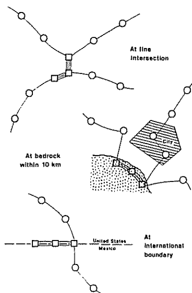
Figure 2-10.—Network junctions.
