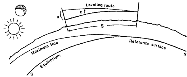
Figure 3-9.—Effect, a , of tidal deflection, \epsilon , on a section of length and direction, \bar{S} .
