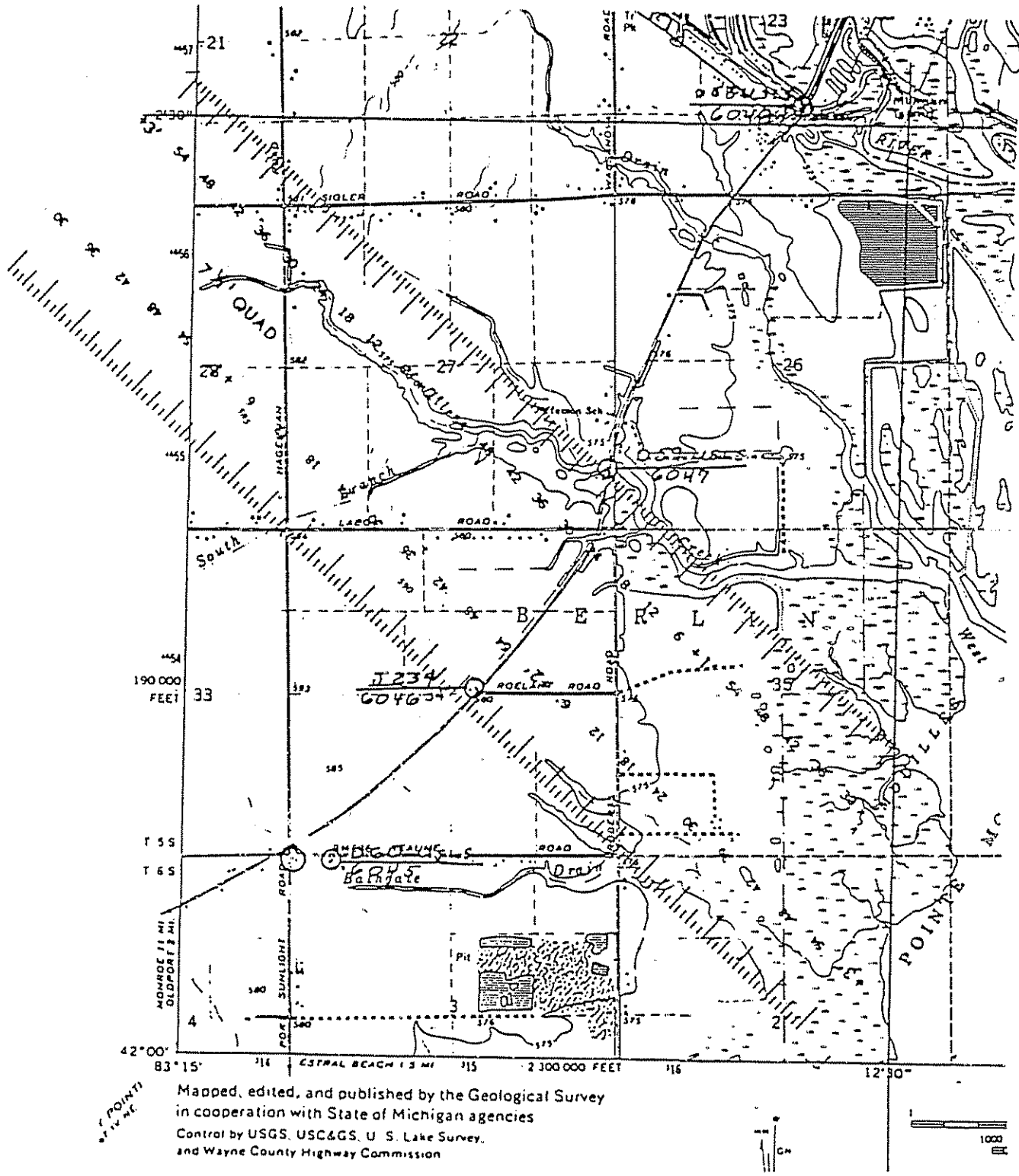
Figure 2-22.—Scaling longitude: D 59 USLS is 83°13'32"W.
