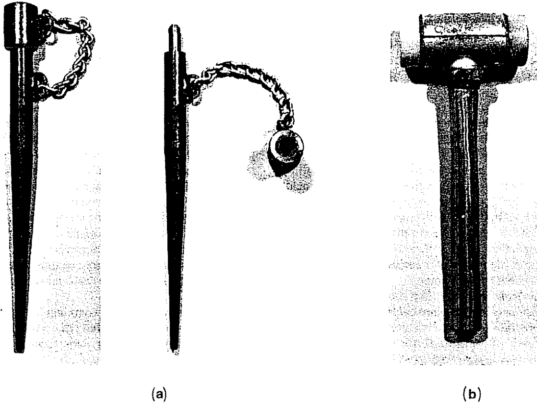
Figure 3-63.—Turning pin (a) and hammer (b).
