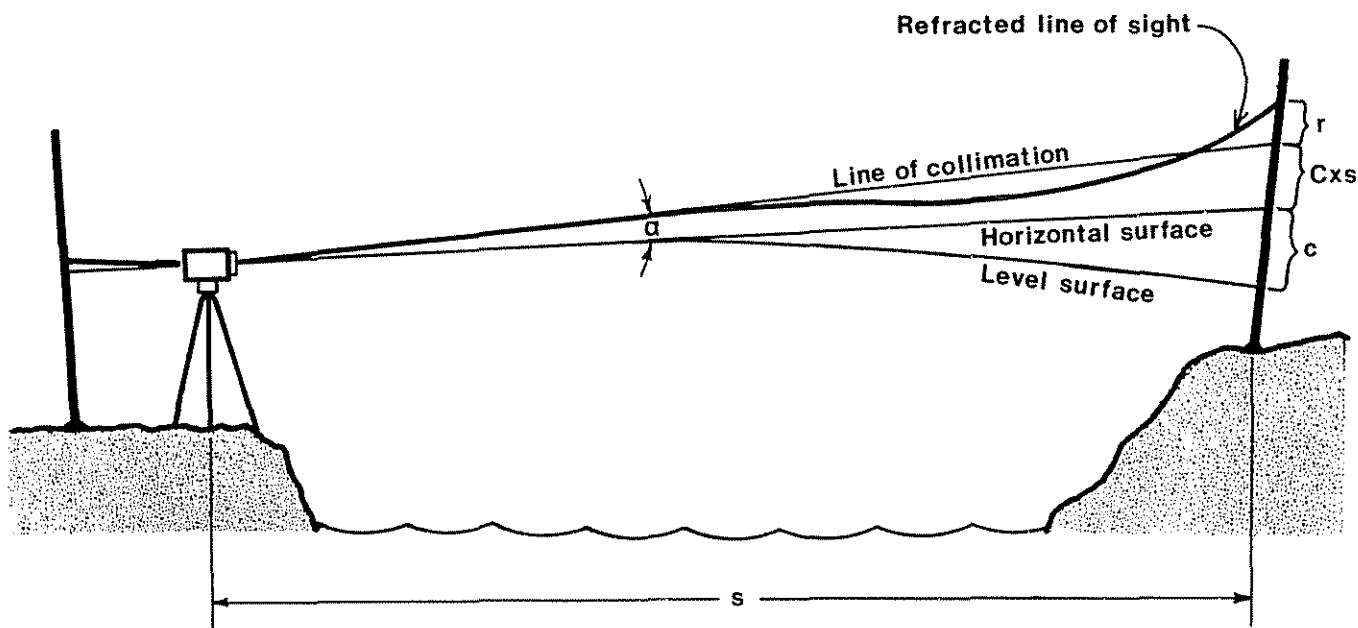
Figure 4-1.—Curvature, c , refraction, r , and the effect, C \times s , of collimation error, \alpha , are magnified by a long sighting distance.
