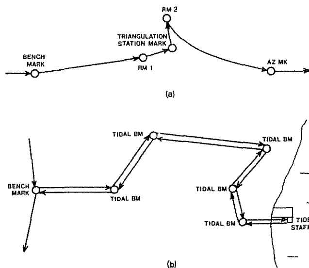
Figure 3-75.—Leveling routes through a cluster of control points at a triangulation station (a) and a tide station (b).
